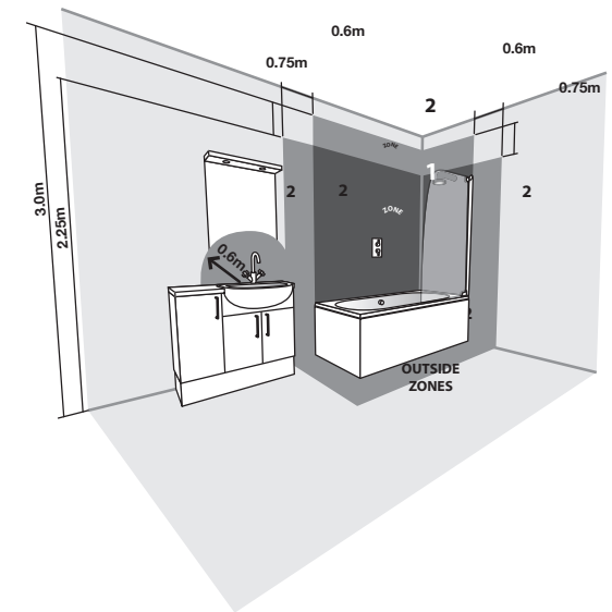
IEE BATHROOM ZONES DIAGRAM
