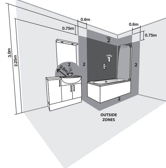
IEE BATHROOM ZONES DIAGRAM
